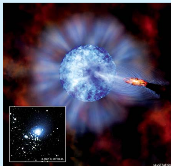
Illustration: NASA/CXC/M. Weiss; X-ray: NASA/CXC/CIA/P. Plucinsky et al.; Optical: NASA/STScI/SDSU/J. Orosz et al.
